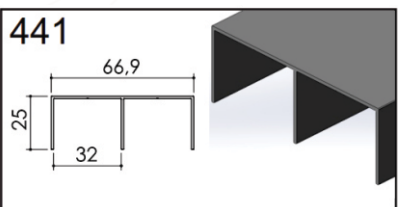
NATURAL OR ANODIZED TOP RAIL DOUBLE 32MM
