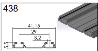
NATURAL OR ANODIZED DOUBLE 29mm RAIL
