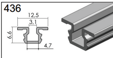
NATURAL SIMPLE RAIL
