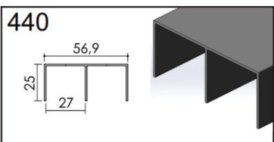
NATURAL OR ANODIZED TOP RAIL DOUBLE 27MM
