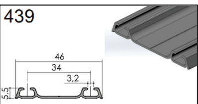
NATURAL OR ANODIZED DOUBLE 34mm RAIL
